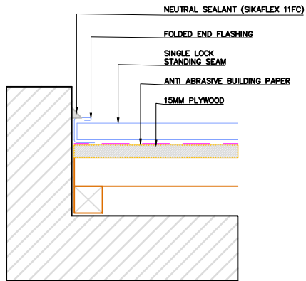
JUNCTION AT WALL – HORIZONTAL
