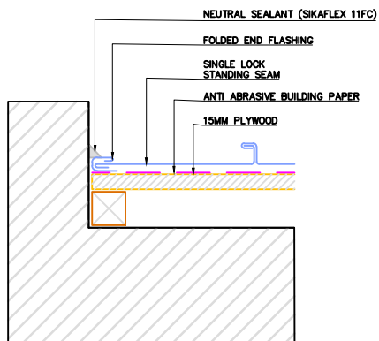
JUNCTION AT WALL – VERTICAL
